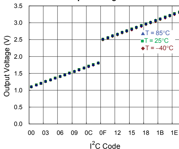
LDO2 Output Voltage vs. I 2 C Code
