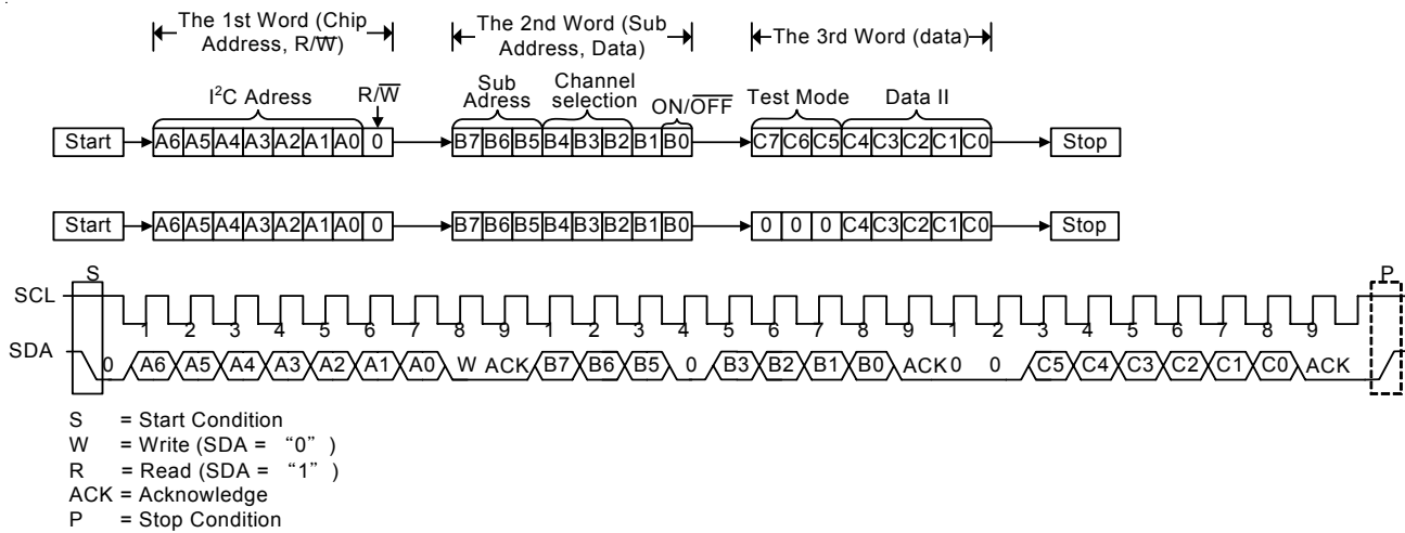
Figure 1. I²C Interface Trimming Diagram
