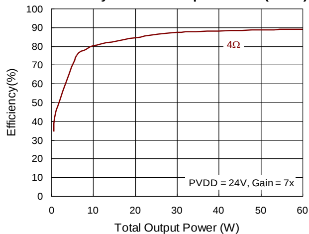
Efficiency vs. Total Output Power (PBTL)
