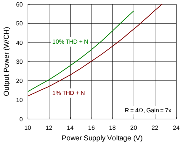
Output Power vs. Power Supply Voltage (PBTTL)
