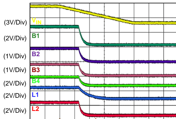
Power Off Sequence
