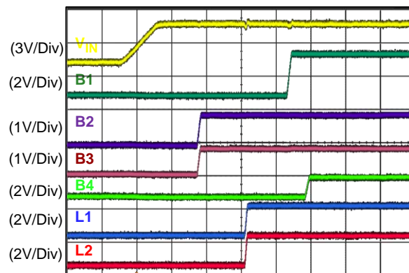
Power Up Sequence for GPIO3 = Hiz
