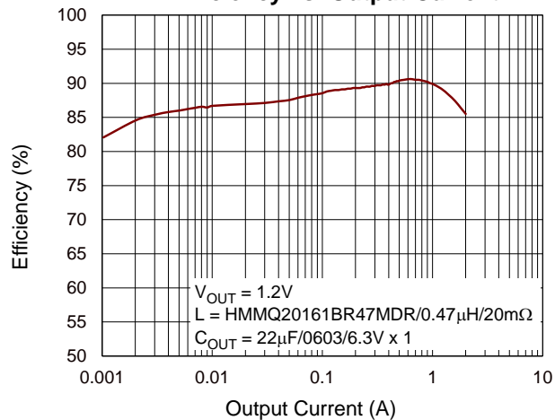
B4 Efficiency vs. Output Current
