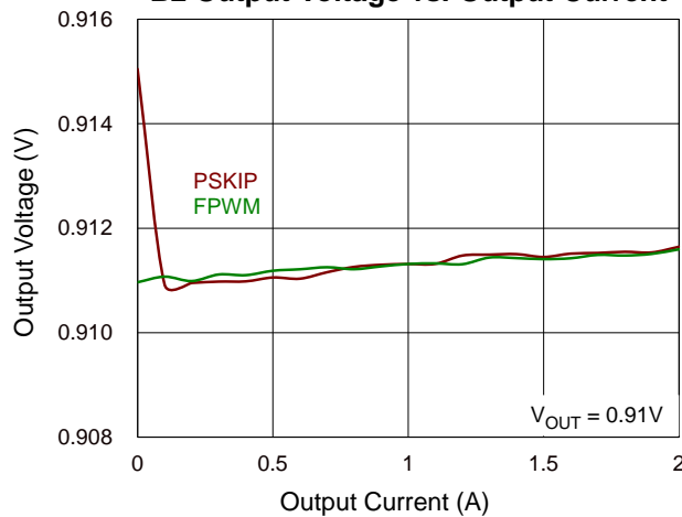
B2 Output Voltage vs. Output Current
