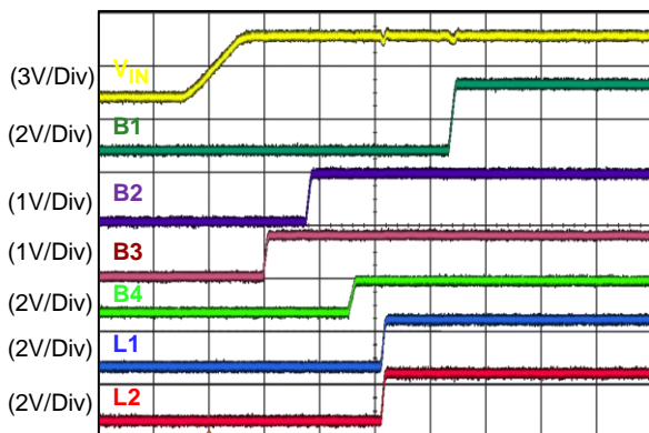
Power Up Sequence for GPIO3 = L
