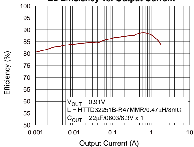
B2 Efficiency vs. Output Current
