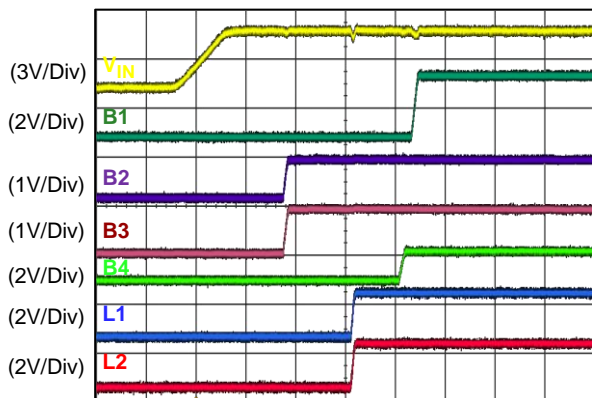
Power Up Sequence for GPIO3 = H
